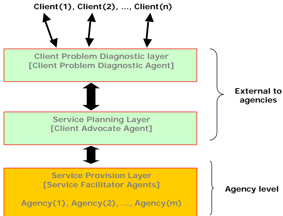
Figure 1. The ServiceNet Framework
