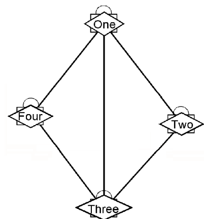
Figure 3. Reduced graph
